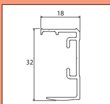
Ram - u-lister
