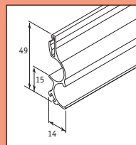
Underlist profil
