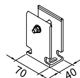
track bracket for track-only fixture
