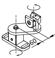
universal track bracket 100 mm
